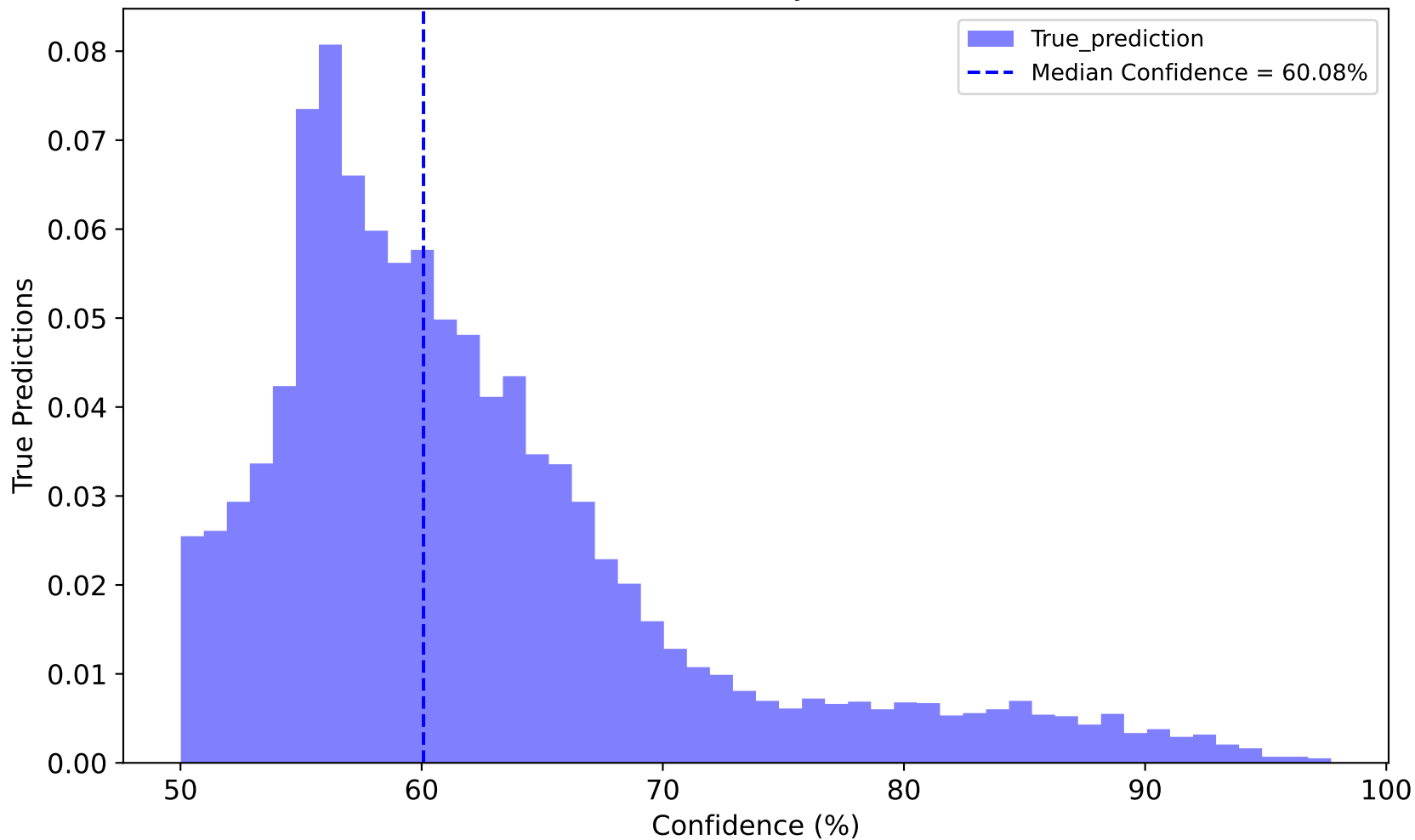
Confidence for Binary Classification
